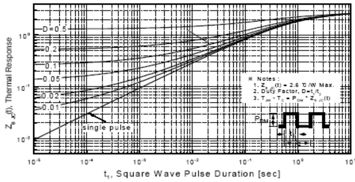
Figure 11-2. Transient Thermal Response Curve for PMS8N65F
