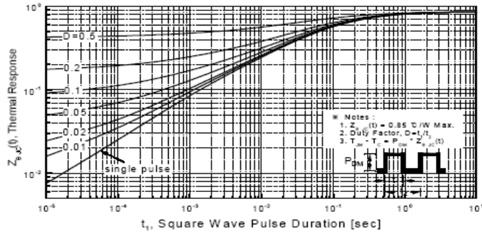
Figure 11-1. Transient Thermal Response Curve for PMS8N65P
