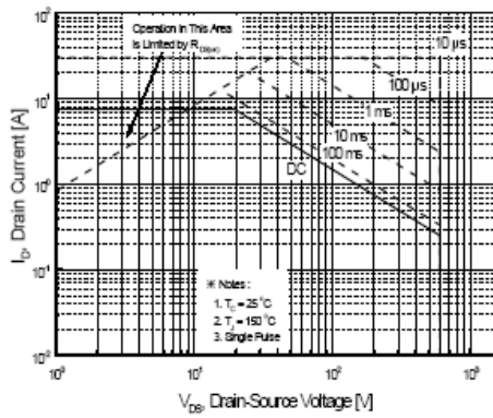
Figure 9-1. Maximum Safe Operating Area for PMS8N65P
