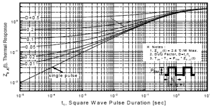
Figure 11-2. Transient Thermal Response Curve for PMS8N60P
