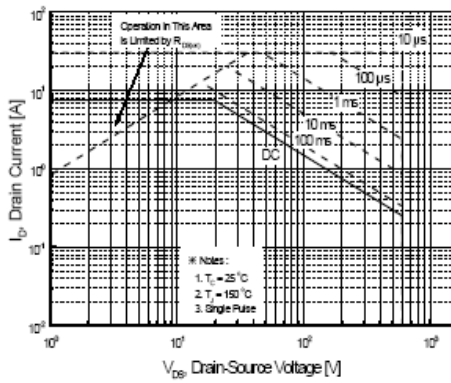
Figure 9-1. Maximum Safe Operating Area for PMS8N60P
