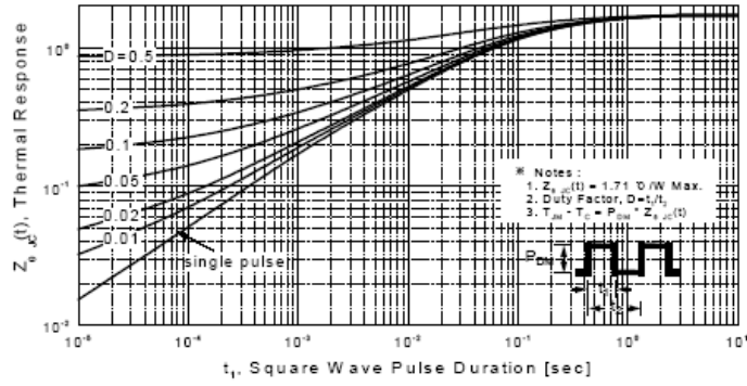
Figure 11-1. Transient Thermal Response Curve for PMS830P
