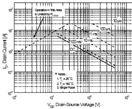
Figure 9-1. Maximum Safe Operating Area for PMS830P
