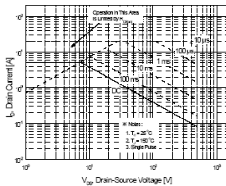
Figure 9-2. Maximum Safe Operating Area for PMS830F
