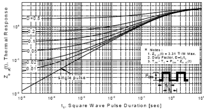
Figure 11-2. Transient Thermal Response Curve for PMS830F
