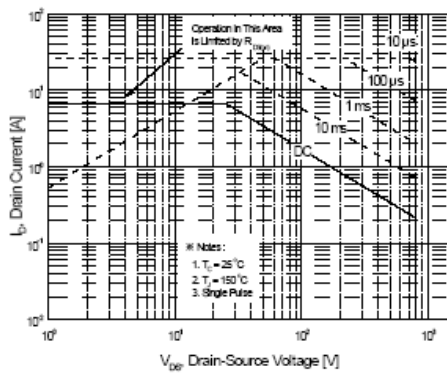
Figure 9-1. Maximum Safe Operating Area for PMS7N80P
