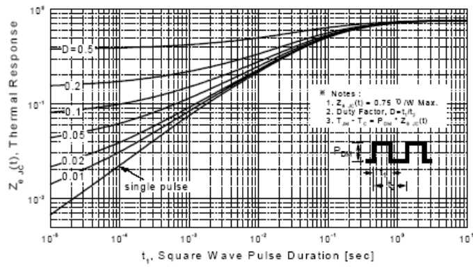
Figure 11-1. Transient Thermal Response Curve for PMS7N80P
