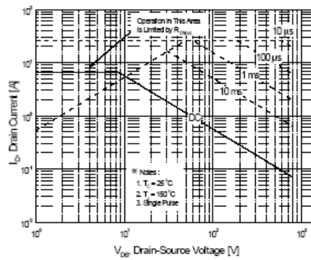
Figure 9-2. Maximum Safe Operating Area for PMS7N80F
