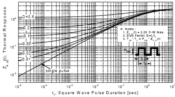
Figure 11-2. Transient Thermal Response Curve for PMS7N80F
