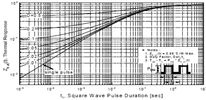
Figure 11-1. Transient Thermal Response Curve for PMS7N60P
