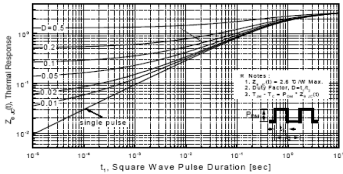
Figure 11-2. Transient Thermal Response Curve for PMS7N60F
