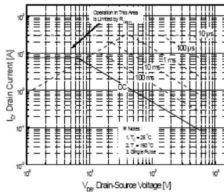
Figure 9-2. Maximum Safe Operating Area for PMS7N60F
