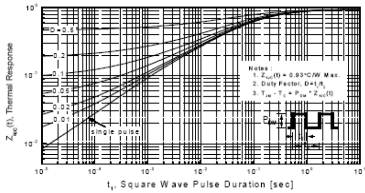
Figure 11-1. Transient Thermal Response Curve for PMS740P
