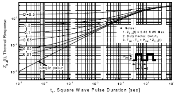
Figure 11-2. Transient Thermal Response Curve for PMS740F
