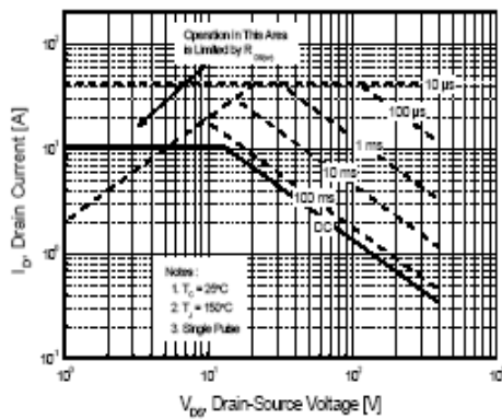
Figure 9-1. Maximum Safe Operating Area for PMS740P
