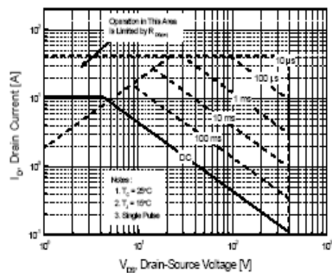
Figure 9-2. Maximum Safe Operating Area for PMS740F
