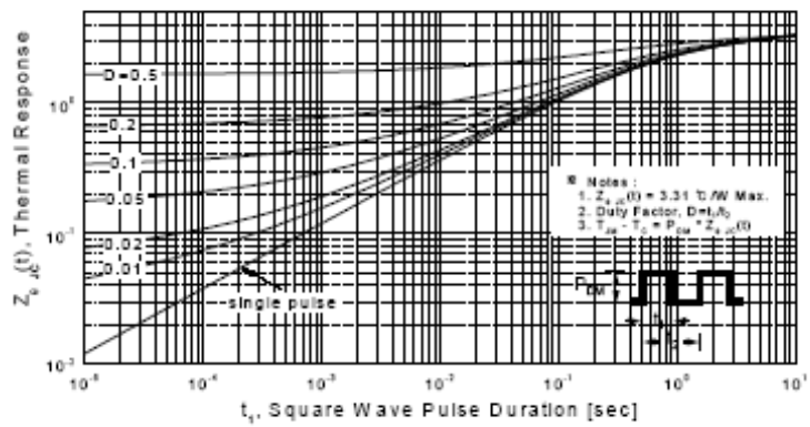
Figure 11-2. Transient Thermal Response Curve for PMS730F
