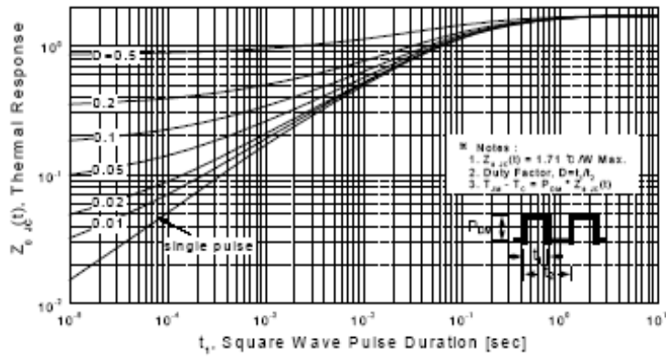
Figure 11-1. Transient Thermal Response Curve for PMS730P
