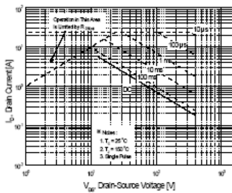
Figure 9-1. Maximum Safe Operating Area for PMS730P
