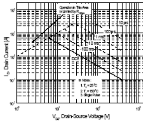
Figure 9-2. Maximum Safe Operating Area for PMS730F
