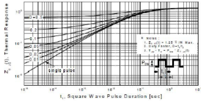
Figure 11-1. Transient Thermal Response Curve for PMS5N65P
