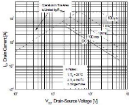
Figure 9-1. Maximum Safe Operating Area for PMS5N65P
