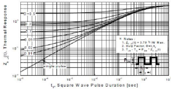
Figure 11-2. Transient Thermal Response Curve for PMS5N65F
