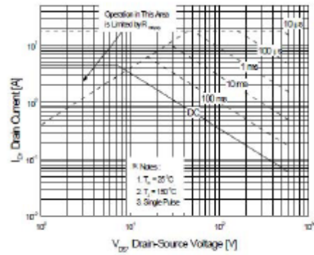
Figure 9-2. Maximum Safe Operating Area for PMS5N65F
