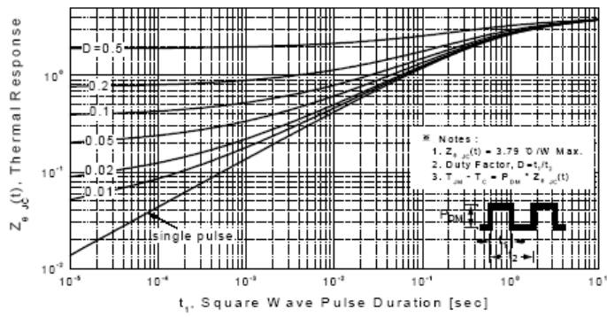
Figure 11-2. Transient Thermal Response Curve for PMS5N60F
