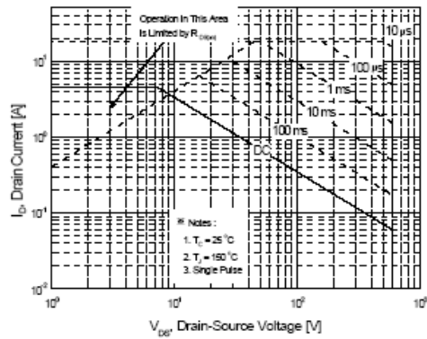
Figure 9-2. Maximum Safe Operating Area for PMS5N60F
