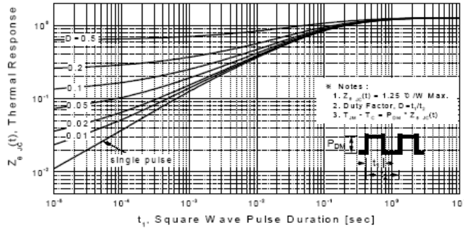
Figure 11-1. Transient Thermal Response Curve for PMS5N60P
