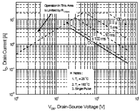
Figure 9-1. Maximum Safe Operating Area for PMS5N60P
