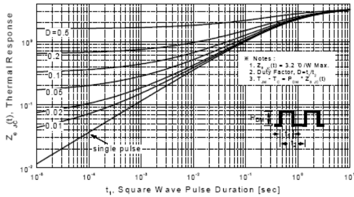
Figure 11-2. Transient Thermal Response Curve for PMS3N80F
