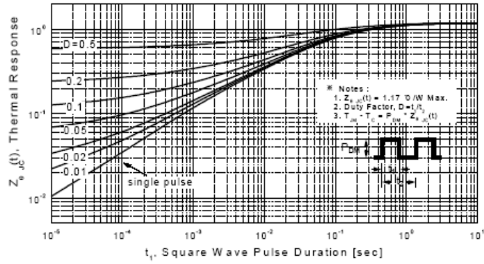
Figure 11-1. Transient Thermal Response Curve for PMS3N80P
