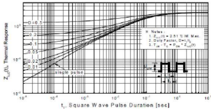
Figure 11-2. Transient Thermal Response Curve for PMS32N20F
