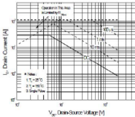
Figure 9-1. Maximum Safe Operating Area for PMS32N20P
