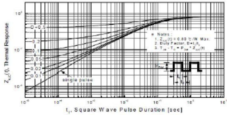
Figure 11-1. Transient Thermal Response Curve for PMS32N20P
