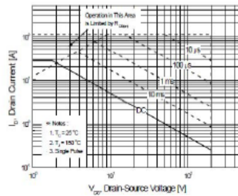
Figure 9-2. Maximum Safe Operating Area for PMS32N20F
