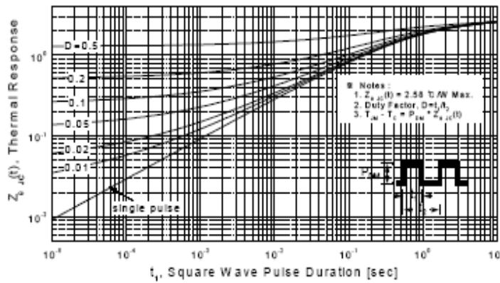
Figure 11-2. Transient Thermal Response Curve for PMS13N50F
