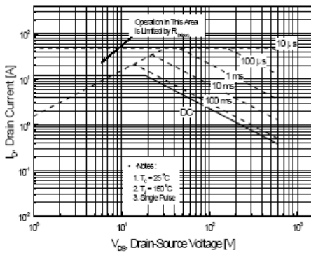
Figure 9-1. Maximum Safe Operating Area for PMS12N60P
