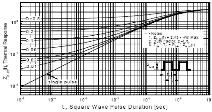
Figure 11-2. Transient Thermal Response Curve for PMS12N60F
