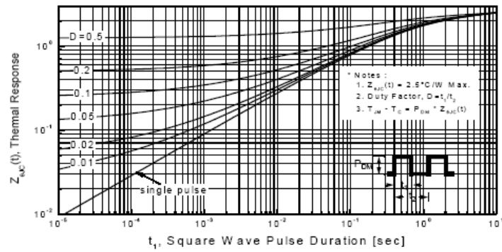
Figure 11-2. Transient Thermal Response Curve for PMS10N65F
