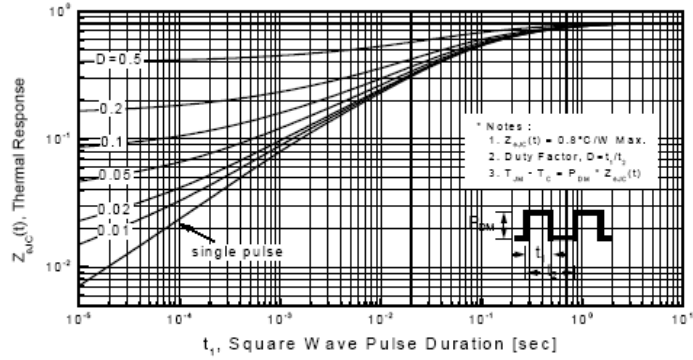
Figure 11-1. Transient Thermal Response Curve for PMS10N65P
