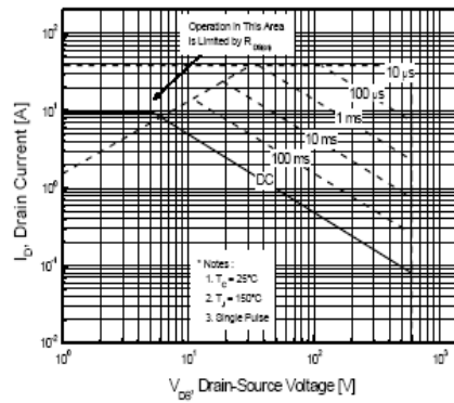
Figure 9-2. Maximum Safe Operating Area for PMS10N65F
