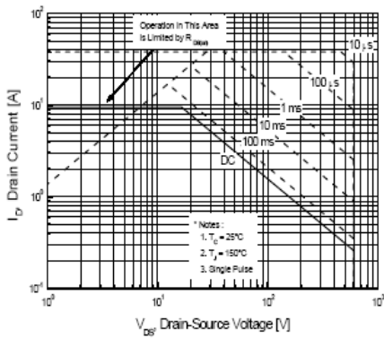
Figure 9-1. Maximum Safe Operating Area for PMS10N60P
