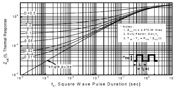
Figure 11-2. Transient Thermal Response Curve for PMS10N60F
