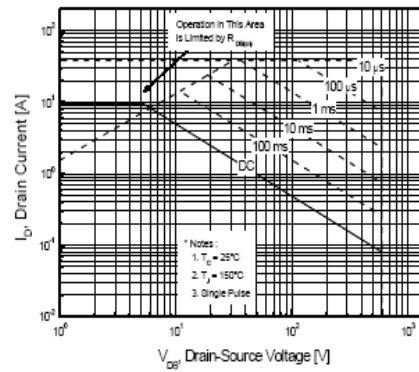
Figure 9-2. Maximum Safe Operating Area for PMS10N60F
