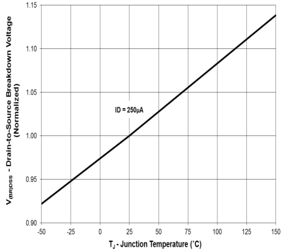
Drain-to-Source Breakdown Voltage vs. Junction Temperature
